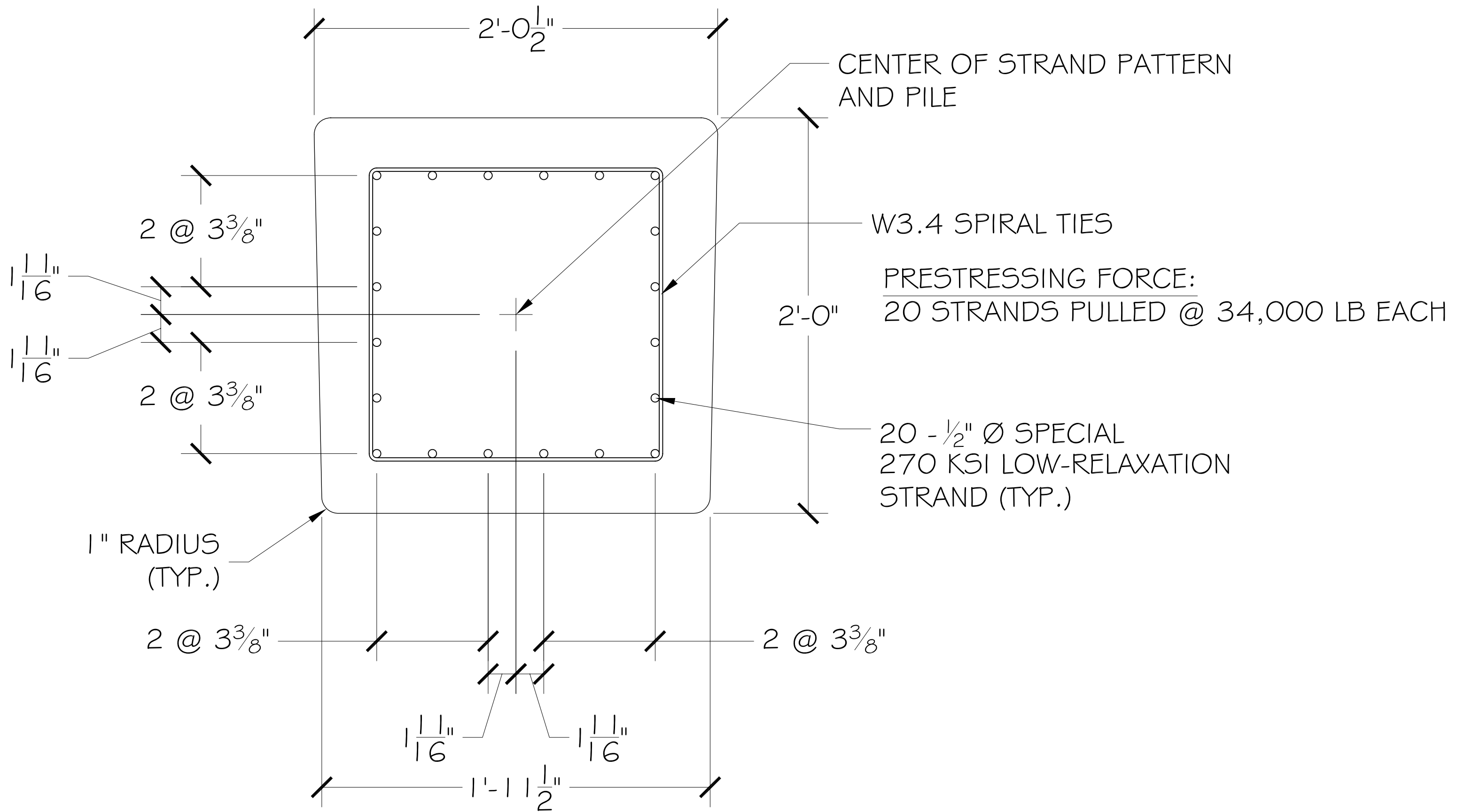
24" x 24" PILE CROSS-SECTION
