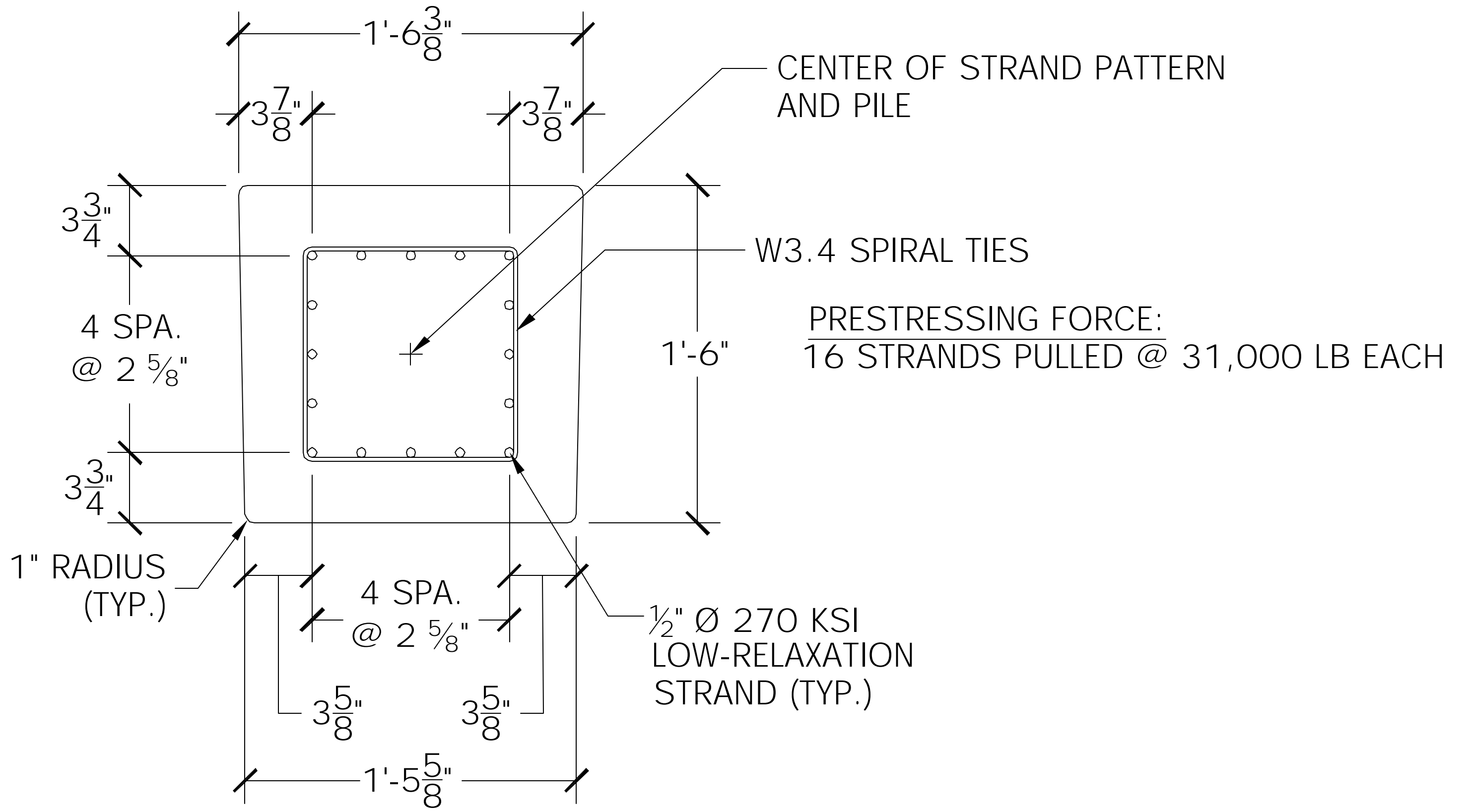
18" x 18" PILE CROSS-SECTION
