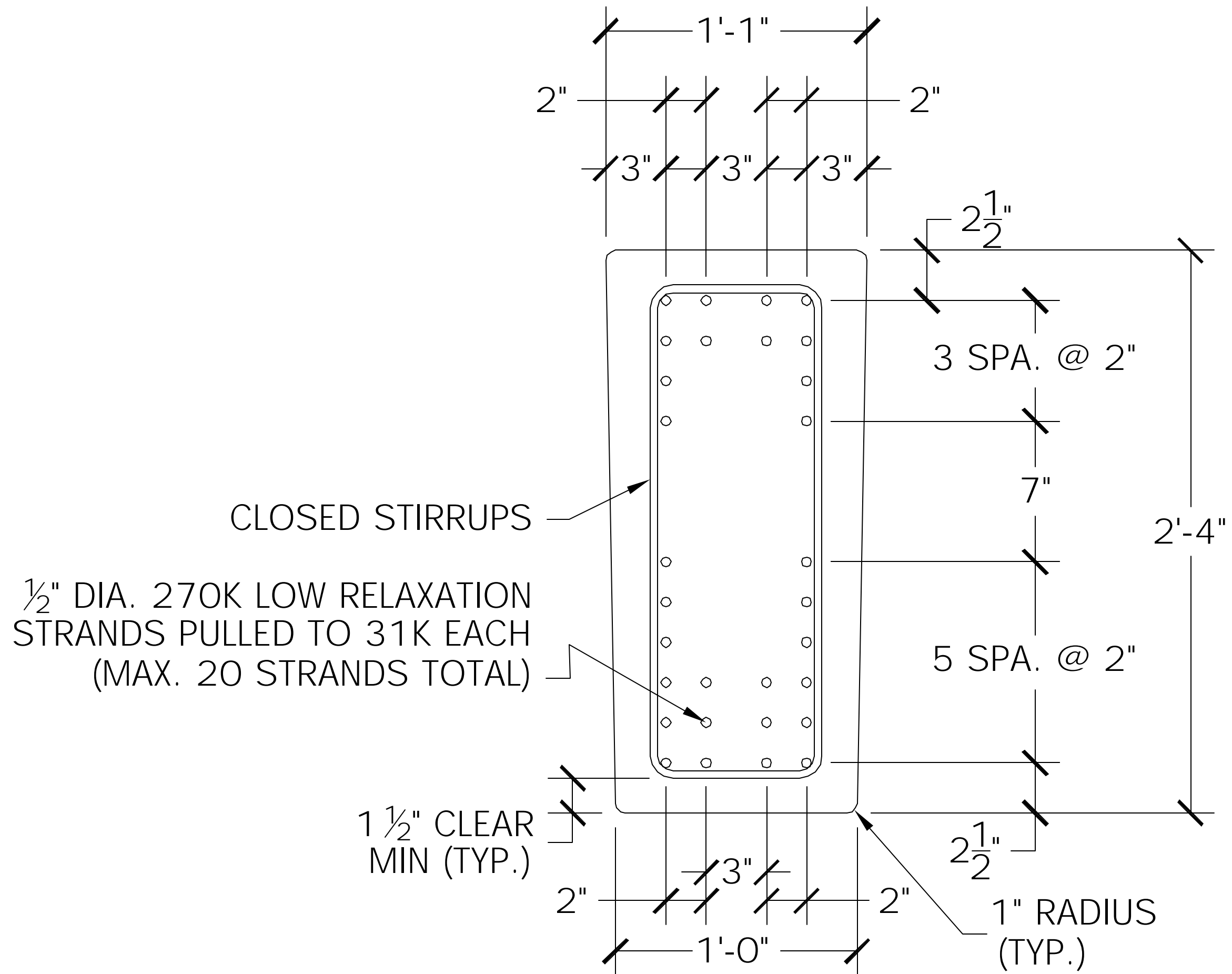
12" x 28" BEAM CROSS-SECTION
