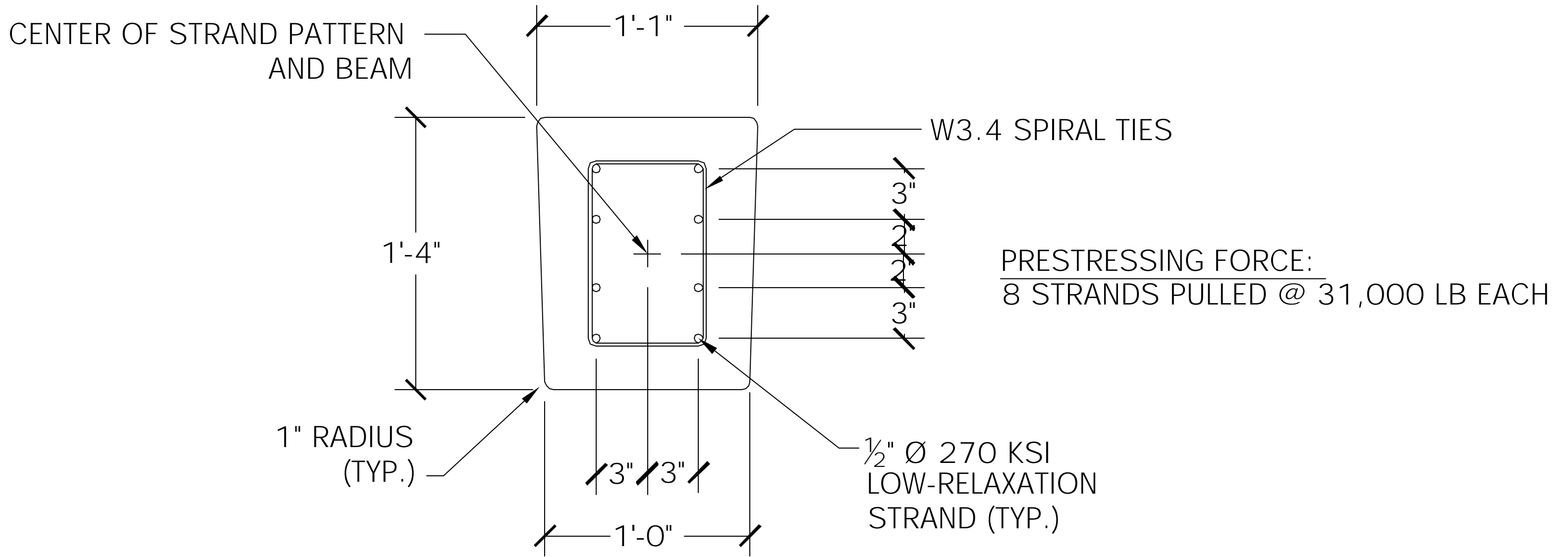
12" x 16" BEAM CROSS-SECTION
